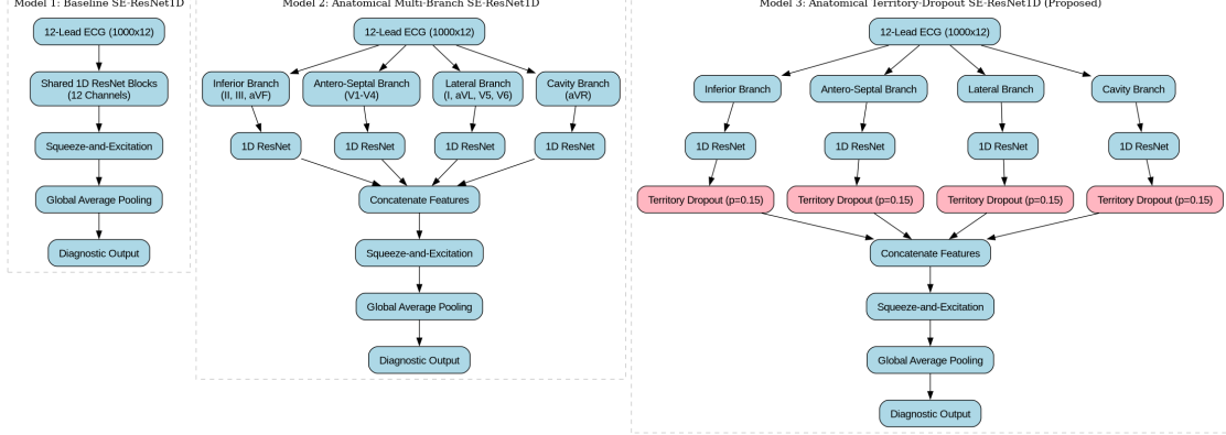
Figure 2: Conceptual architectural progression from Model 1 (Baseline) to Model 2 (Anatomical Multi-Branch) and Model 3 (Anatomical Territory-Dropout).
