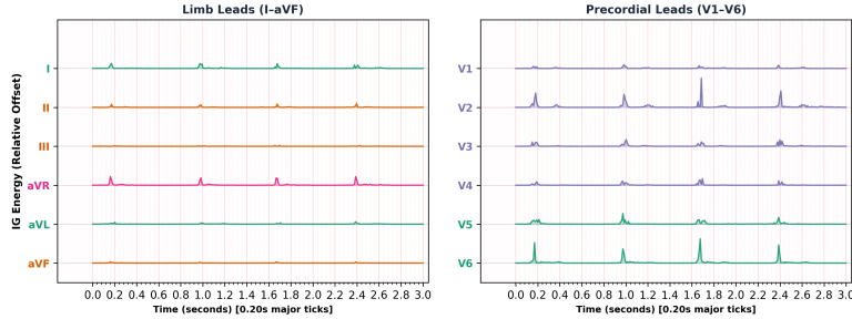
B: Axiomatic Integrated Gradients (Lead-Wise Instantaneous Attribution Energy | Synchronized 3.0s Zoom)
